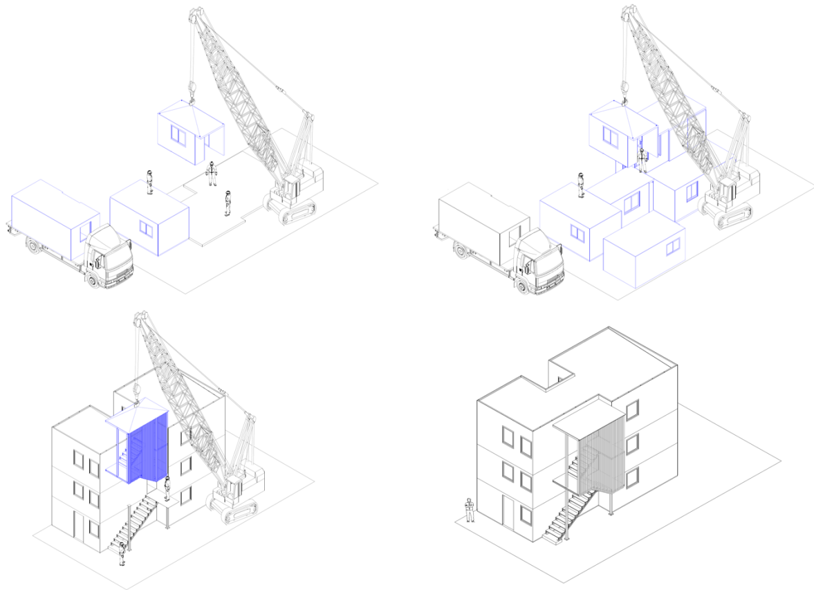
Figure 6. Assembly sequence.
