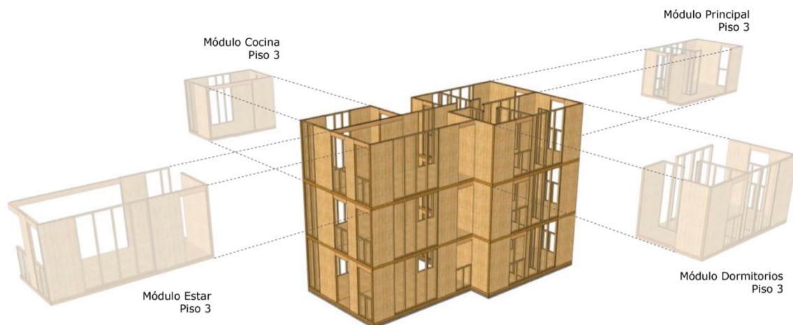
Figure 2. Distribution of the 4 modules per floor.
