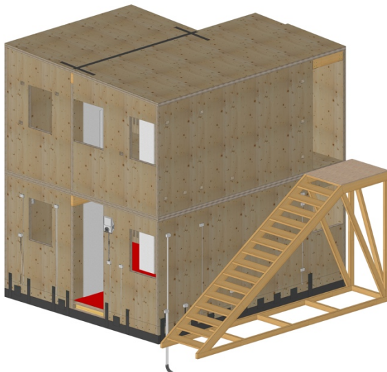
Figure 3. The mockup Model
